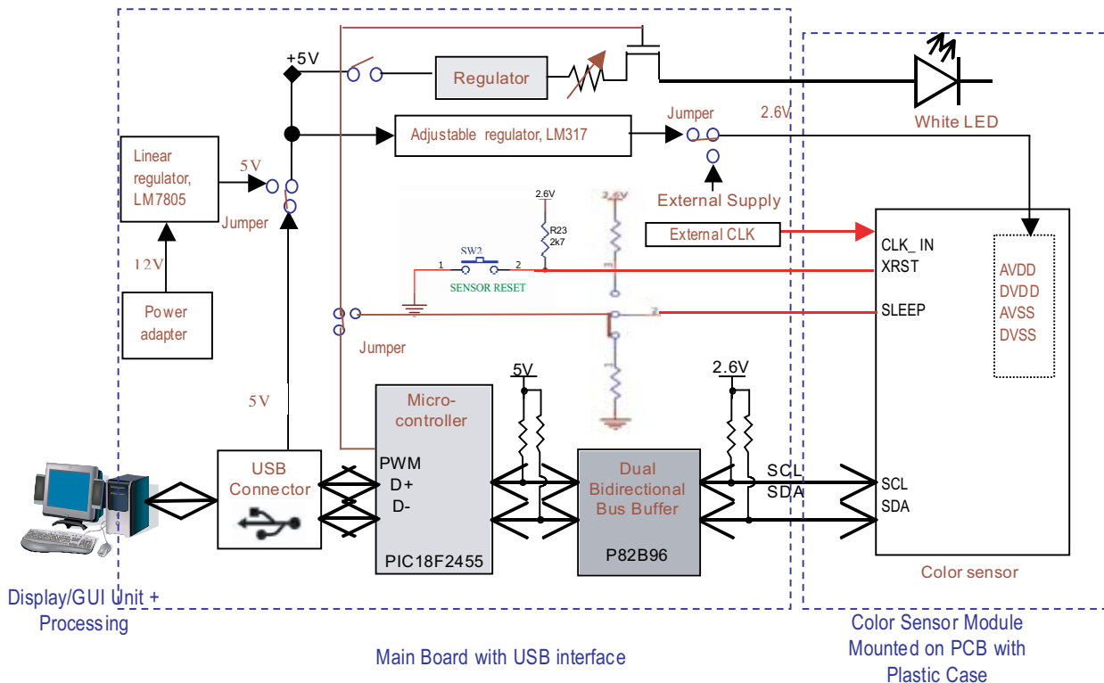
HDJD-JD07 Block Diagram
